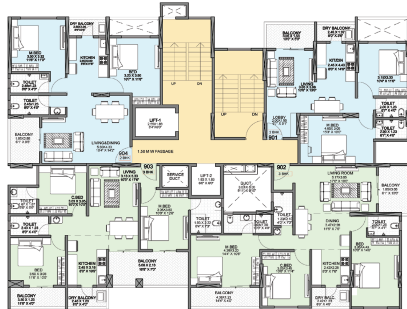
9TH FLOOR PLAN
