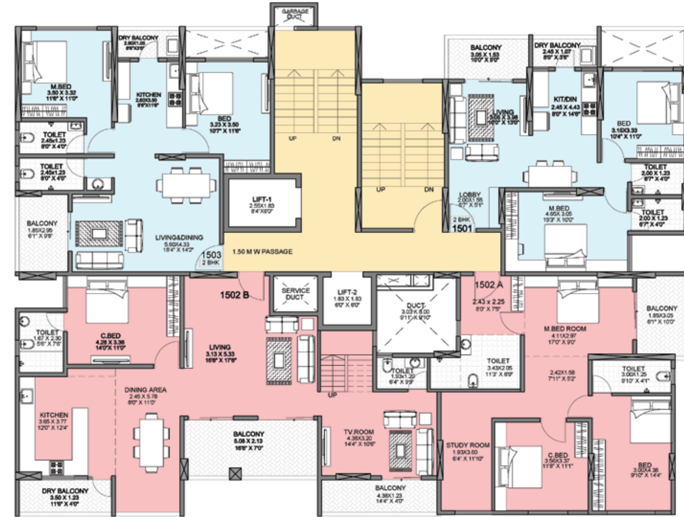
15 M ROAD 15TH FLOOR PLAN
