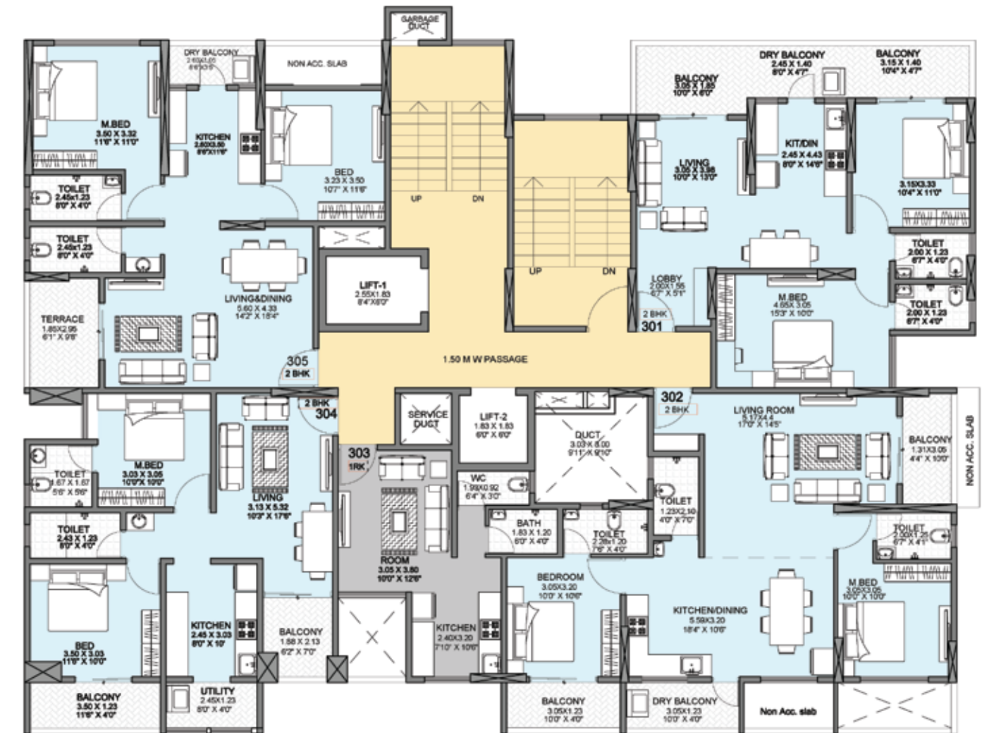
15 M ROAD 3RD FLOOR PLAN
