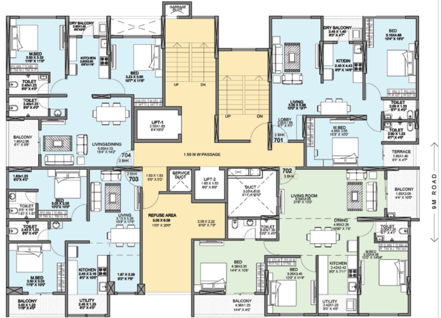
7TH FLOOR PLAN
