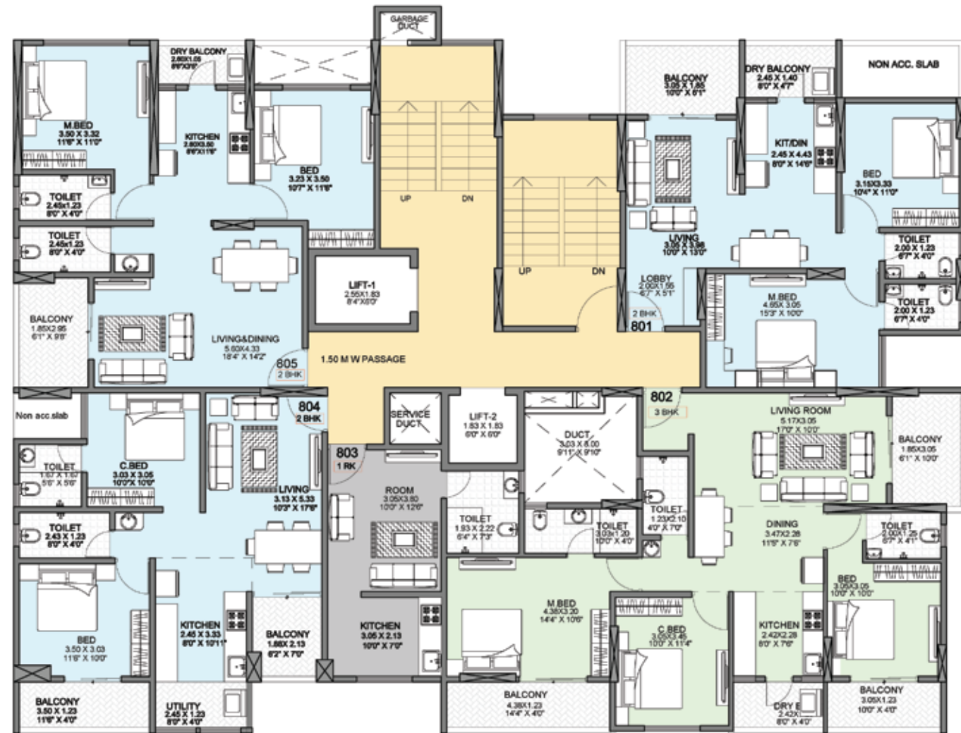
8TH FLOOR PLAN
