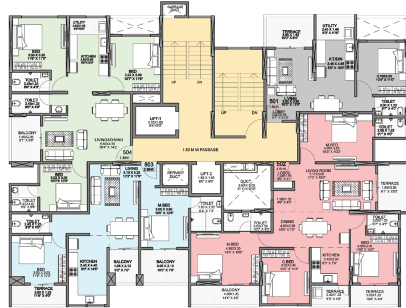
5TH FLOOR PLAN
