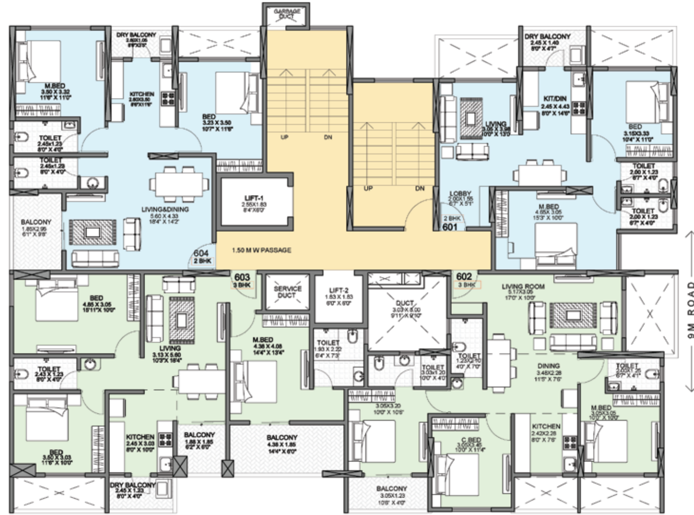
6TH FLOOR PLAN
